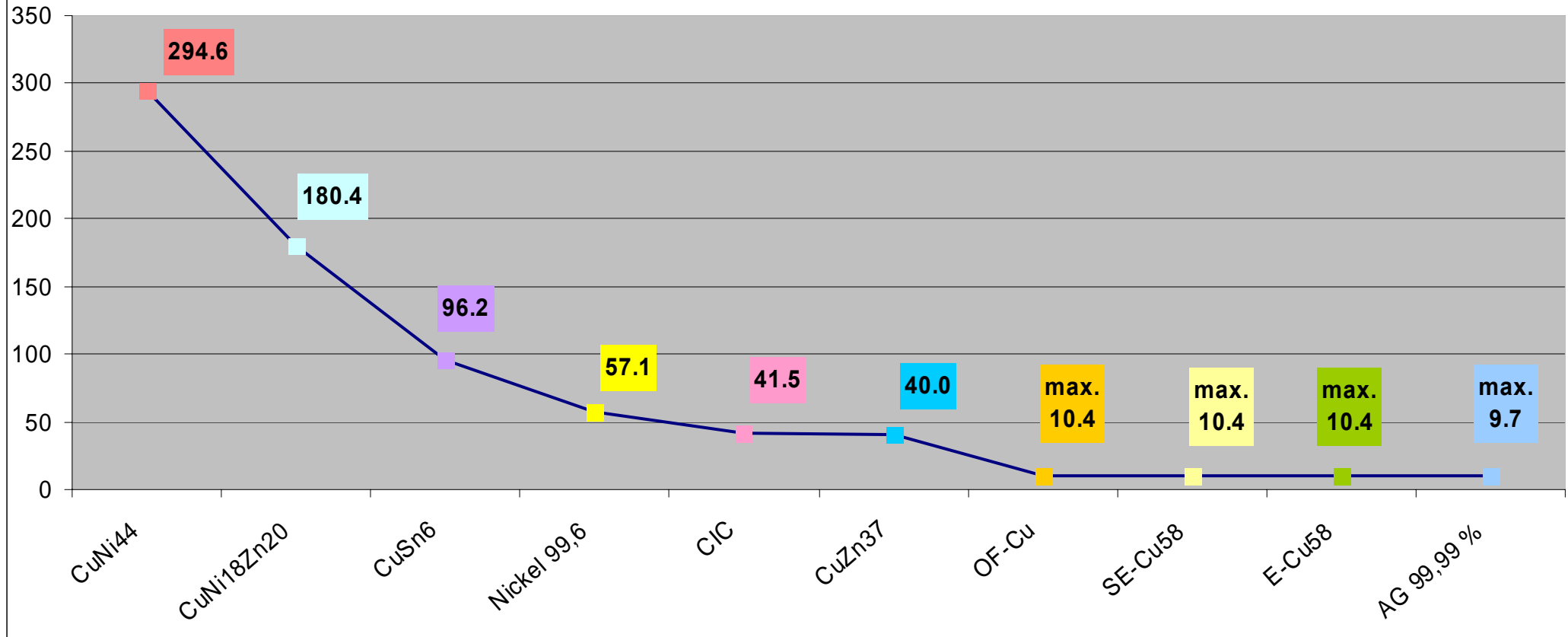
Electrical resistivity \Omega circ. mil/ft.
